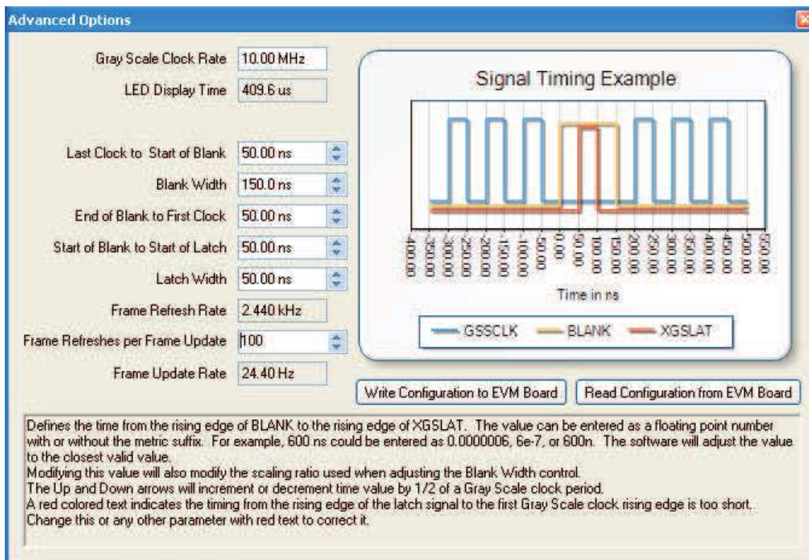
Figure 2. Advanced Options
