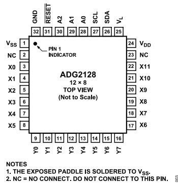
Figure 3. Pin Configuration
