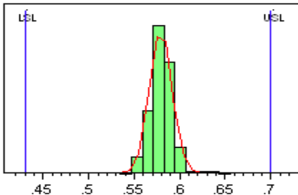
Figure 3. VGG at 1.95 GHz, VDD=4V; IDD= 50mA
