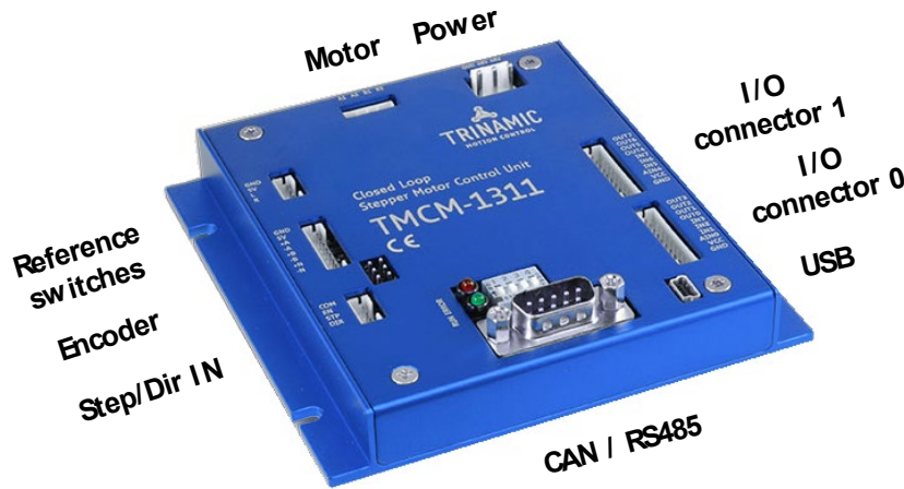
Figure 3.2 TMCM-1311 connectors
