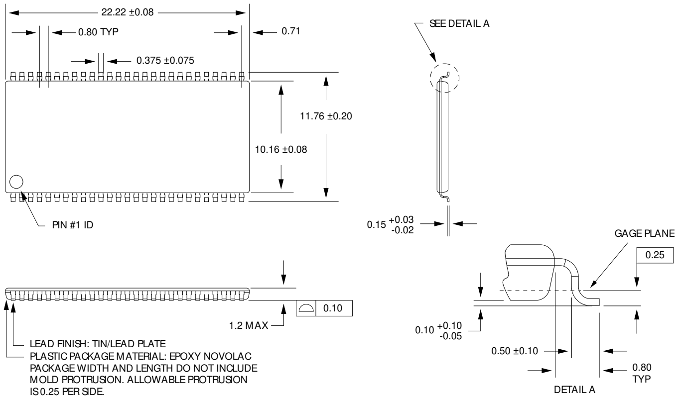
Figure 59: 54-Pin Plastic TSOP (400 mil)
