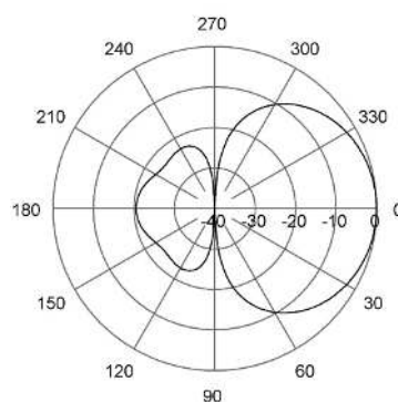
E-Plane | 405 MHz
