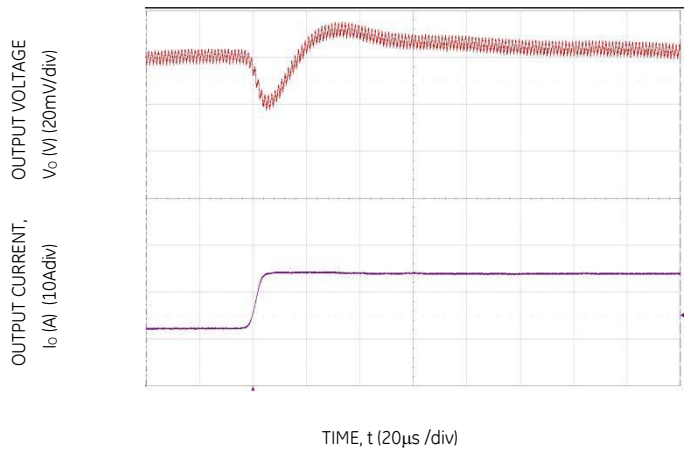
Figure 22. Transient Response to Dynamic Load Change from 50% to 100% at 12Vin, Cout = 2x47uF+1x330uF, CTune=3300pF & RTune=240Ω
