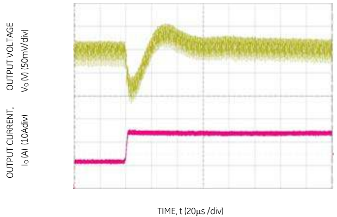
Figure 34. Transient Response to Dynamic Load Change from 50% to 100% at 12Vin, C_{out} = 1 \times 47 \mu\text{F} + 1 \times 330 \mu\text{F} , C_{Tune}=2200\text{pF} & R_{Tune}=300\Omega
