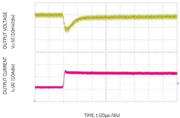
Figure 10. Transient Response to Dynamic Load Change from 50% to 100% at 12Vin, C out = TBD, CT tune =TBD & RT tune =TBD
