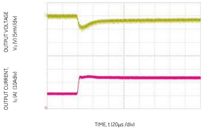
Figure 4. Transient Response to Dynamic Load Change from 50% to 100% at 12V in , C out =1x47uF+11x330uF, C Tune =47nF, R Tune =180Ω
