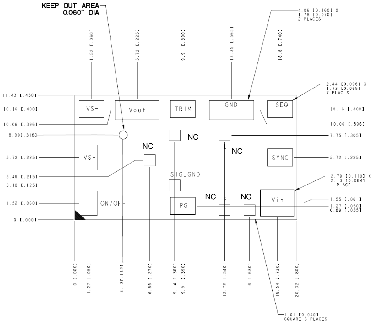
RECOMMENDED FOOTPRINT - THROUGH THE BOARD -
