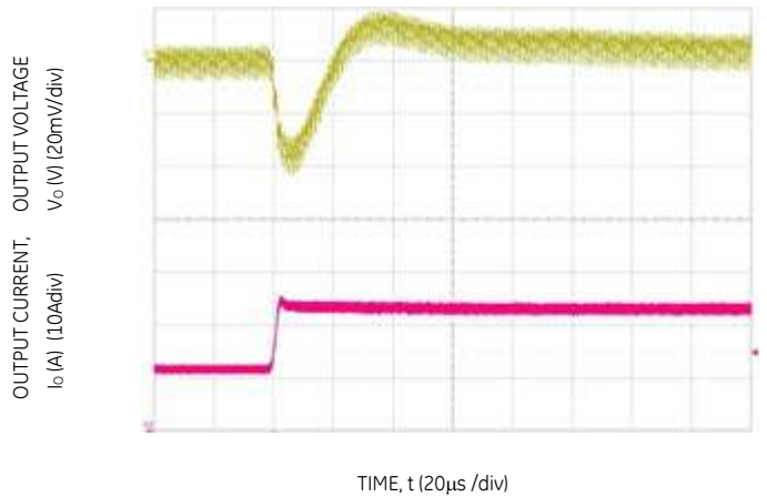
Figure 16. Transient Response to Dynamic Load Change from 50% to 100% at 12Vin, C_{out}= \text{TBD} , C_{Tune}= \text{TBD} & R_{Tune}= \text{TBD}
