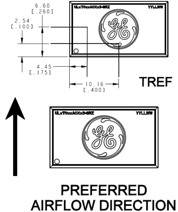
Figure 48. Preferred airflow direction and location of hot-spot of the module ( T_{ref} ).
