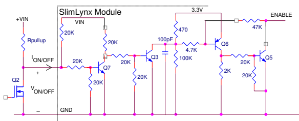
Figure 39. Circuit configuration for using positive On/Off logic.
