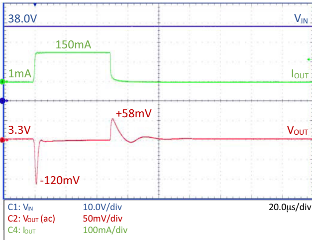
Figure 20. Load Transient – NCV8730–3.3 V, C_{OUT} = 1\text{ }\mu\text{F}
