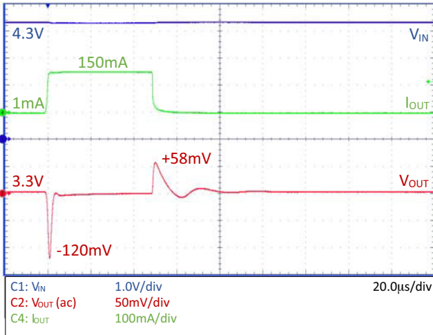
Figure 18. Load Transient – NCV8730–3.3 V, C_{OUT} = 1\text{ }\mu\text{F}
