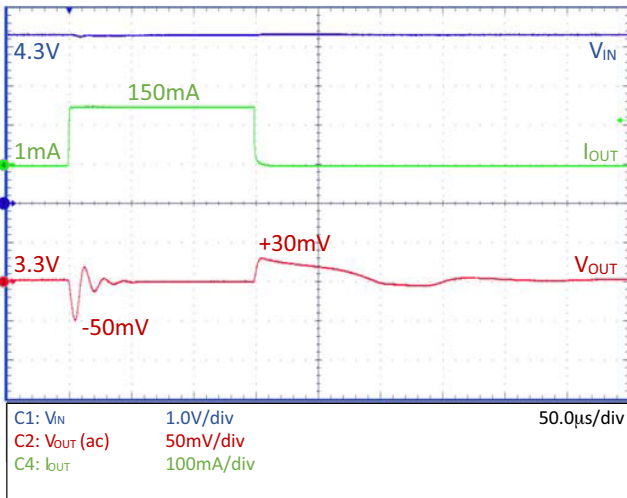
Figure 22. Load Transient – NCV8730–3.3 V, C_{OUT} = 22\text{ }\mu\text{F}
