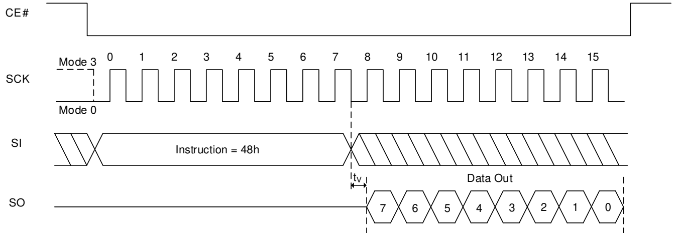
Figure 8.27 Read Function Register Sequence In SPI Mode
