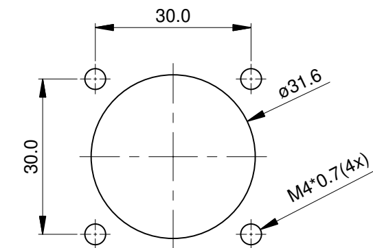
MOUNTING HOLE
