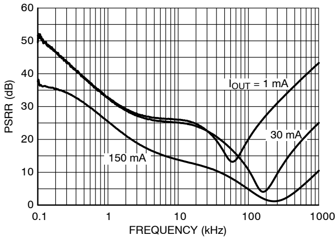
Figure 17. PSRR, 1.5 V Version, V_{IN} = 2.5 V
