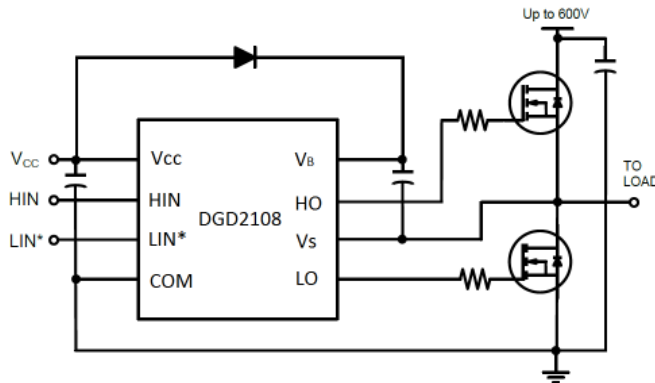
Typical Configuration
