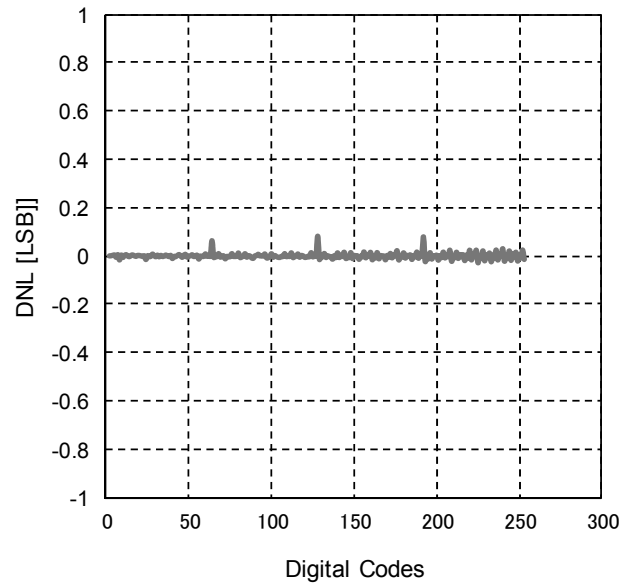
Fig.46 VCOM DNL
