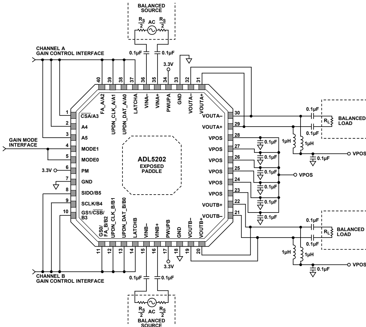
Figure 54. Basic Connections
