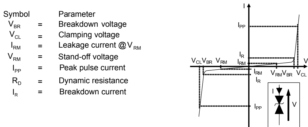
Figure 1. Electrical characteristics (definitions)
