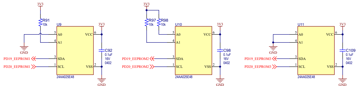
Figure 3-17. EEPROM 24AA025E48
