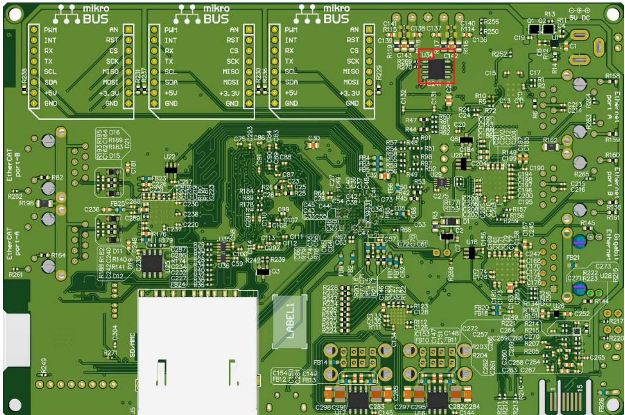
Figure 3-16. ATECC608A Location
