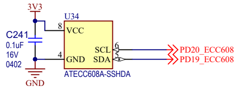
Figure 3-15. ATECC608A-SSHDA Implementation
