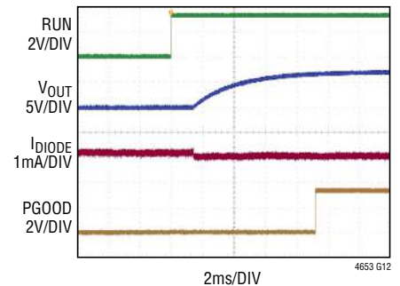
FIGURE 32 CIRCUIT, 48V_{IN} , C_{INH} = C_D = 4.7\mu\text{F} , C_{OUT} = 22\mu\text{F} \times 2 , R_{ISET} = 124\text{k} , R_{ISET} = 240\text{k} , R_{PGDFB} = 95.3\text{k} , C_{TH} = 10\text{nF} , R_{TH} = 562\Omega , R_{EXTVCC} = 49.9\Omega , C_{EXTVCC} = 1\mu\text{F} , V_{OUT} PRE-BIASED TO 5V THROUGH 1N4148 DIODE
