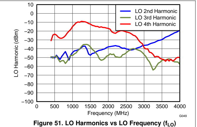
Figure 51. LO Harmonics vs LO Frequency ( f_{LO} )
