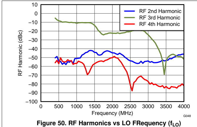
Figure 50. RF Harmonics vs LO Frequency ( f_{LO} )
