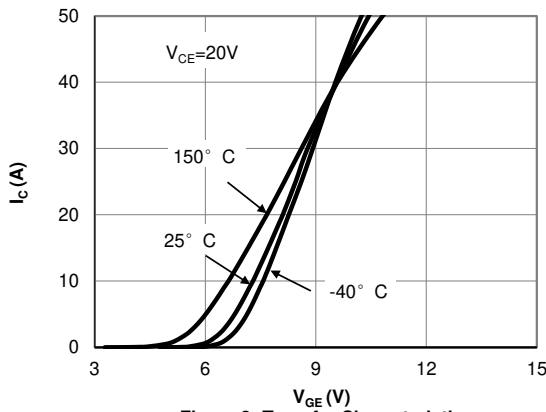
Figure 3: Transfer Characteristic
