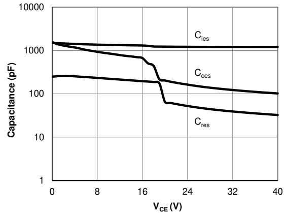
Figure 8: Capacitance Characteristic
