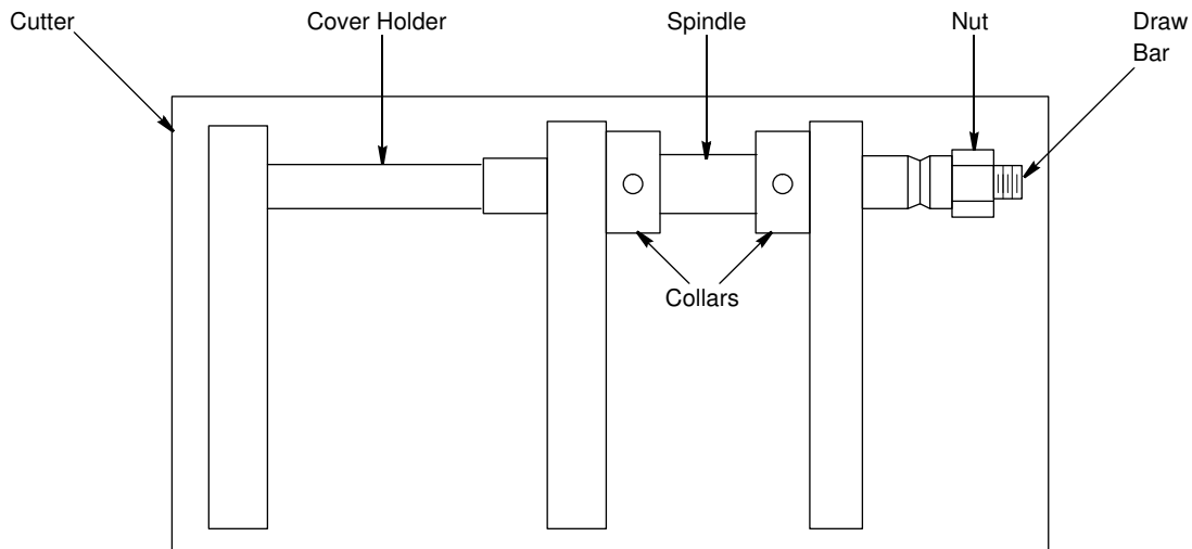
Cutter Replacement
