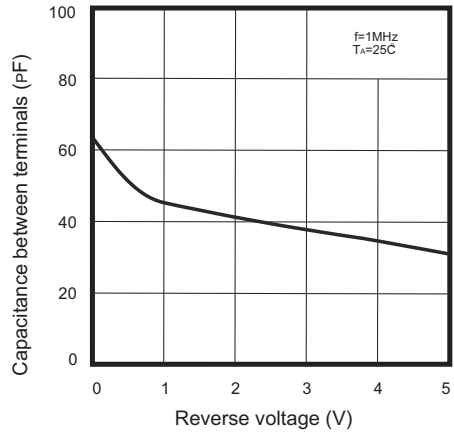
Fig.4 - Capacitance between terminals characteristics
