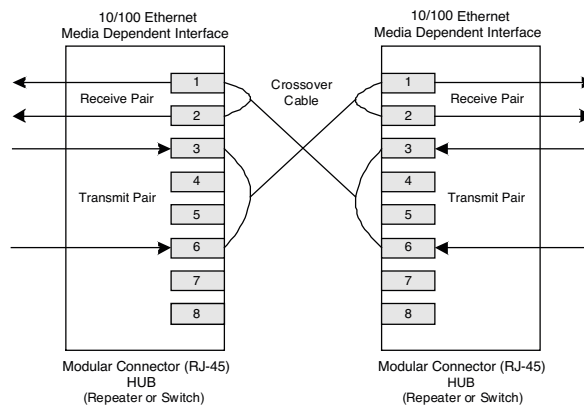
Figure 2. Crossover Cable
