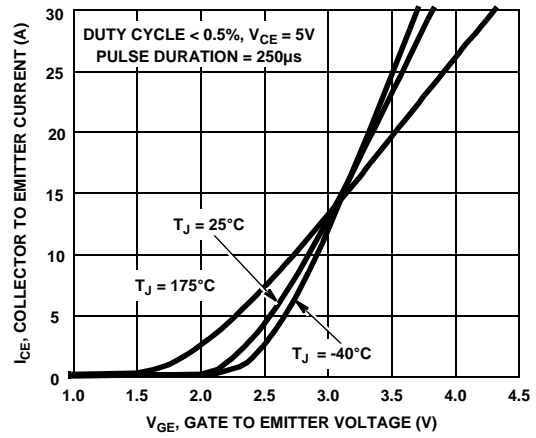
Figure 8. Transfer Characteristics
