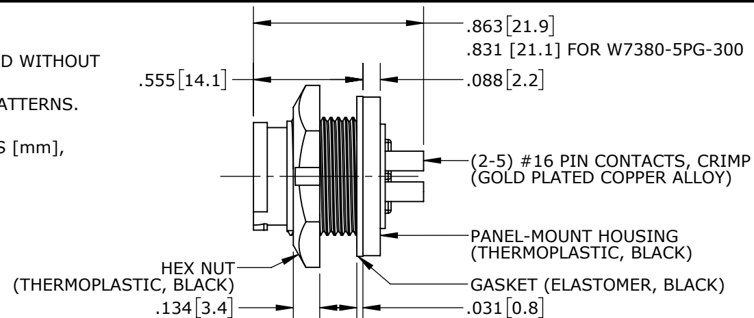
CRIMP CONTACTS (SHOWN ASSEMBLED) W7380-4PG-P-300 SHOWN
