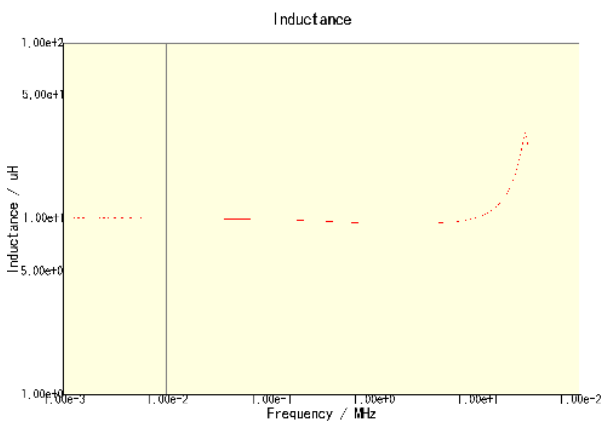
CLF6045T-100M-CA
