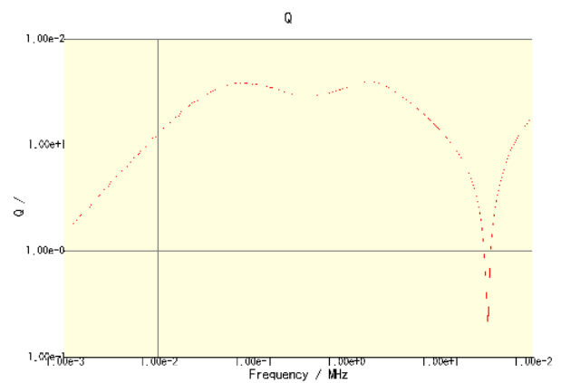
CLF6045T-100M-CA
