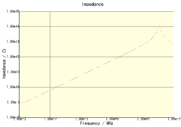
CLF6045T-100M-CA
