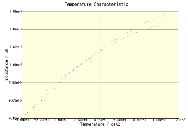
CLF6045T-100M-CA(DC = 0A)
