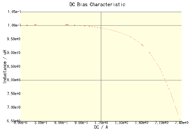
CLF6045T-100M-CA(Amb. Temp. = 20degc)
