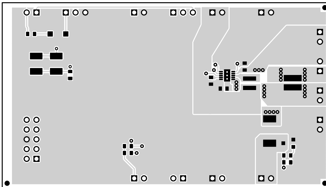
Figure 10. Top Layer
