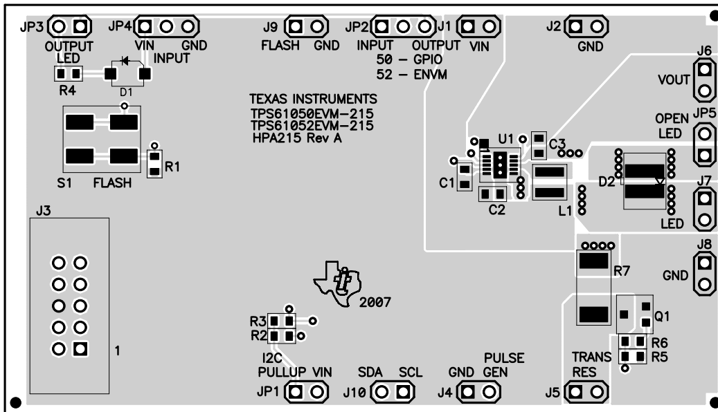
Figure 9. Assembly Layer
