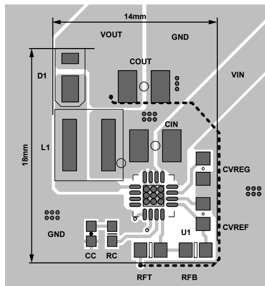
Figure 26. Suggested Layout for 18 mm × 14 mm, +12 V Input to -5 V Output Application (Dashed Line Is Connected on the Internal Layer of the PCB; Other Vias Connected to the Ground Plane; SS, EN, PWRGD, SLEW, and SYNC/FREQ Connections Not Shown for Clarity and Are Typically Connected on an Internal Layer)
