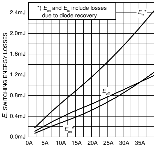
Figure 13. Typical switching energy losses as a function of collector current (inductive load, T_J = 175^\circ\text{C} , V_{CE} = 400\text{V} , V_{GE} = 0/15\text{V} , r_G = 12\Omega , Dynamic test circuit in Figure E)
