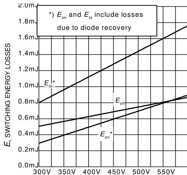
Figure 16. Typical switching energy losses as a function of collector emitter voltage (inductive load, T_J = 175^\circ\text{C} , V_{GE} = 0/15\text{V} , I_C = 20\text{A} , r_G = 12\Omega , Dynamic test circuit in Figure E)
