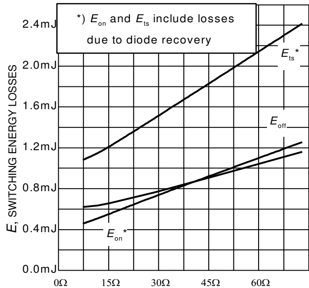
Figure 14. Typical switching energy losses as a function of gate resistor (inductive load, T_J = 175^\circ\text{C} , V_{CE} = 400\text{V} , V_{GE} = 0/15\text{V} , I_C = 20\text{A} , Dynamic test circuit in Figure E)
