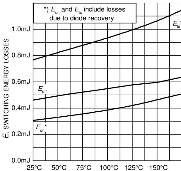
Figure 15. Typical switching energy losses as a function of junction temperature (inductive load, V_{CE} = 400\text{V} , V_{GE} = 0/15\text{V} , I_C = 20\text{A} , r_G = 12\Omega , Dynamic test circuit in Figure E)
