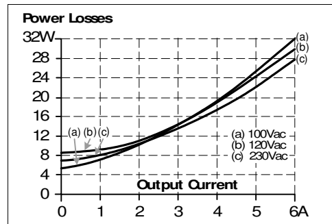
Fig. 8-2 Losses vs. output current at 48V, typ.
