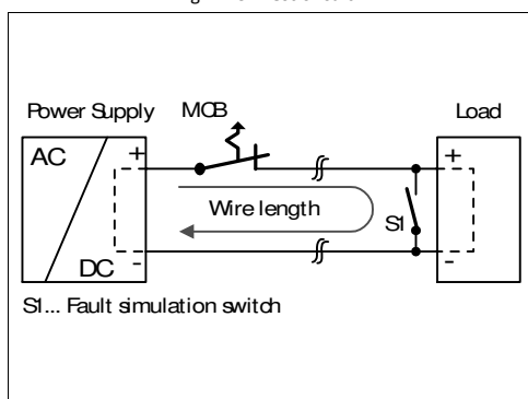
Fig. 22-3 Test circuit
