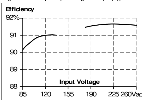
Fig. 8-3 Efficiency vs. input voltage at 48V, 5A, typ.
