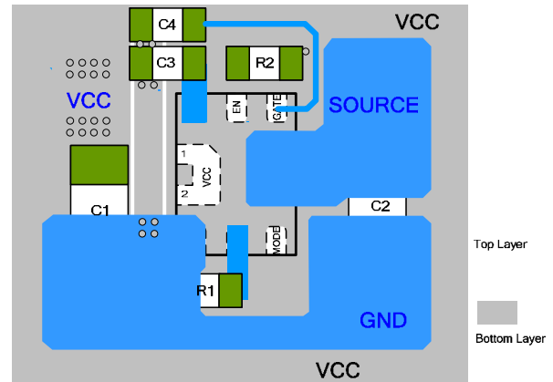
Figure 4: Recommended Layout
