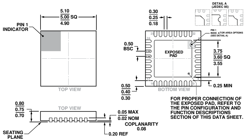
Figure 48. 32-Lead Lead Frame Chip Scale Package [LFCSPP] 5 mm × 5 mm Body and 0.75 mm Package Height (CP-32-12)
