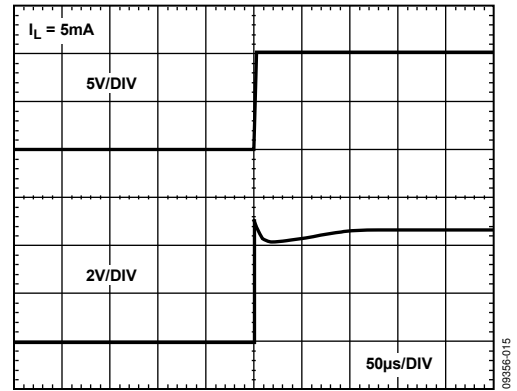
Figure 11. Turn-On Time
