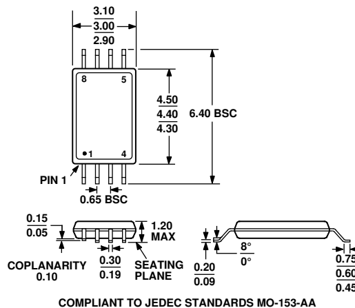
COMPLIANT TO JEDEC STANDARDS MO-153-AA Figure 17. 8-Lead Thin Shrink Small Outline Package [TSSOP] (RU-8) Dimensions shown in millimeters
