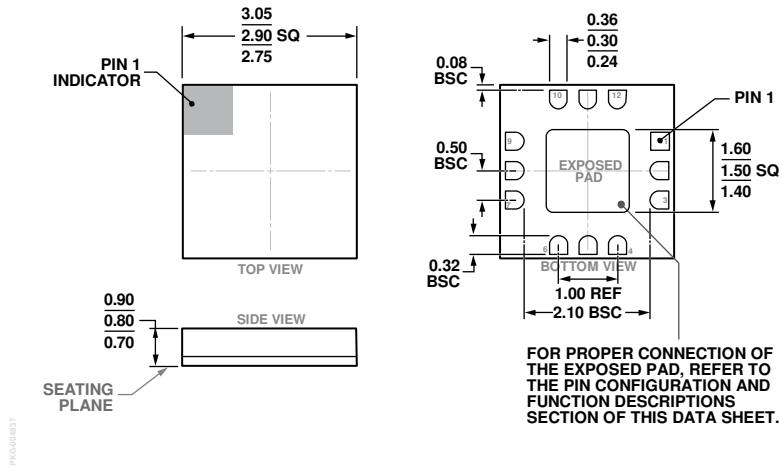
Figure 79. 12-Terminal Ceramic Leadless Chip Carrier [LCC] (E-12-4) Dimensions shown in millimeters
