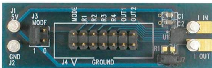
Figure 1. Si85xx-TB Overview (1 kV, 10 Amp Target Board)
