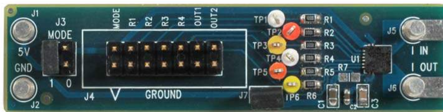
Figure 3. Si85xx20AQFN-TB Overview (1 kV, 20 Amp Target Board)
