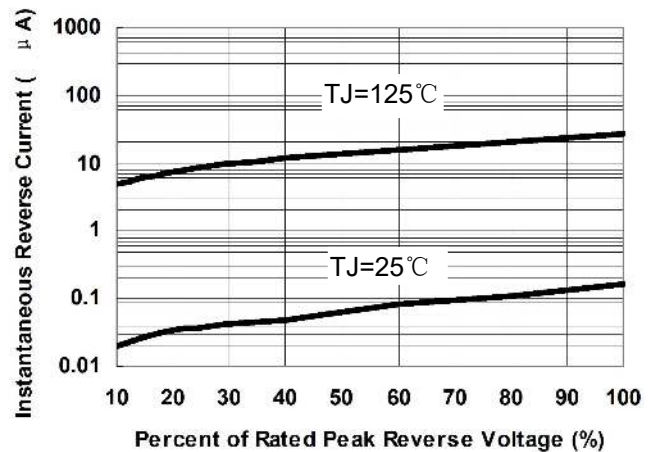
Fig.2-Typical Reverse Characteristics
