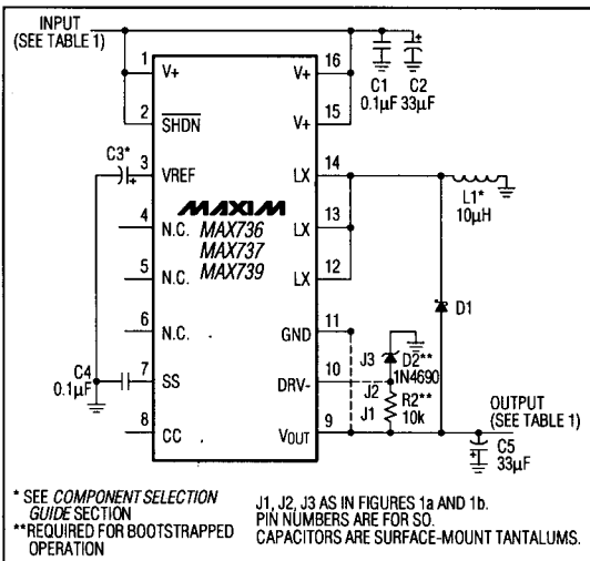
Figure 2. Standard Application Circuit (Surface-Mount Components)
