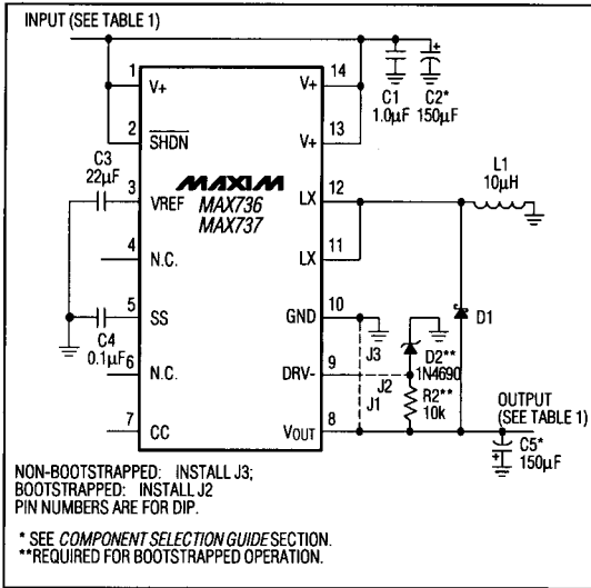
Figure 1a. MAX736/MAX737 Standard Application Circuit (Through-Hole Components)
