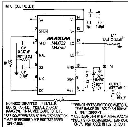
Figure 1b. MAX739/MAX759 Standard Application Circuit (Through-Hole Components)
