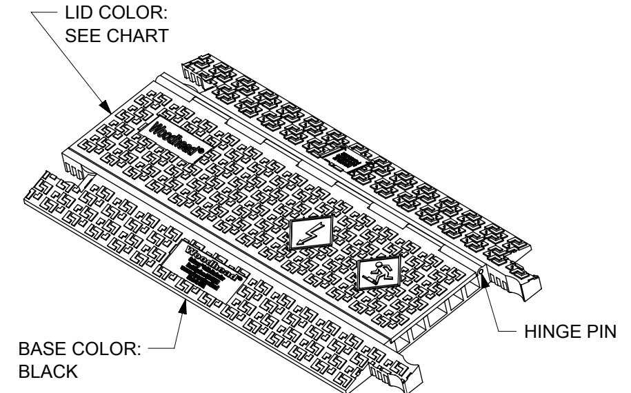
ISOMETRIC VIEWS SCALE 1:10
