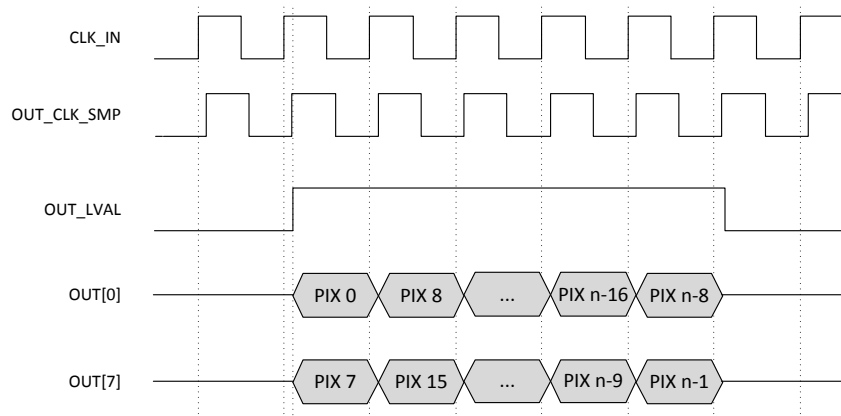
Figure 13: Timing of OUT_CLK_SMP and OUT_LVAL signals
