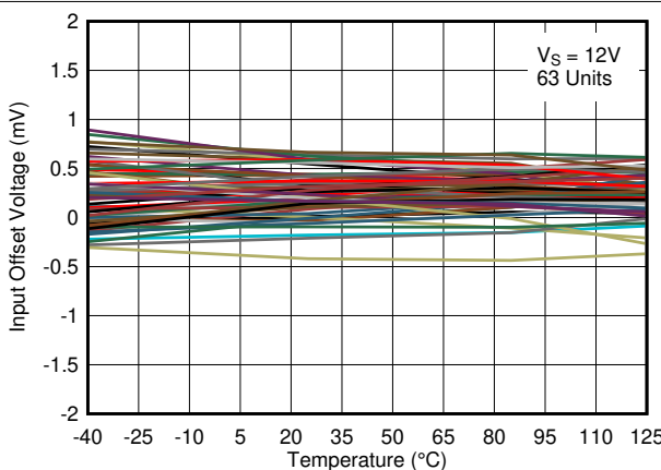
Figure 6-20. Input Offset Voltage vs. Temperature at 12V
