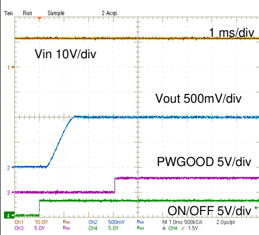
On/Off Enable Delay (Vin=12V, Vout=1.0V, Iout=16A, Cload=660uF)
