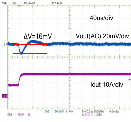
Step Load Transient Response (Vin=12V, Vout=1.0V, Cload=660uF, Iout=8A to 16A 2.4A/us)
