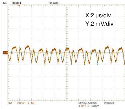
Output Ripple and Noise (Vin=12V, Vout=1.0V, Iout=16A, Cload=660uF, Scope BW=20MHz)
