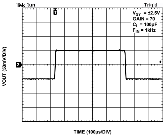
Figure 36. Small Signal Response at C_L = 100 pF and F_{IN} = 1 kHz
