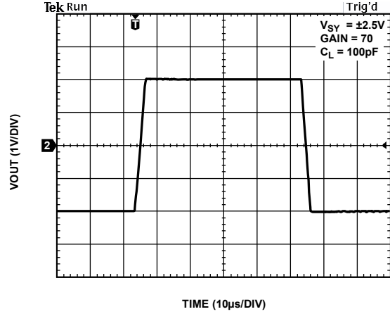
Figure 37. Large Signal Response at C_L = 100 pF
