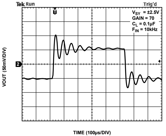
Figure 35. Small Signal Response at C_L = 0.1 \mu F and F_{IN} = 10 kHz
