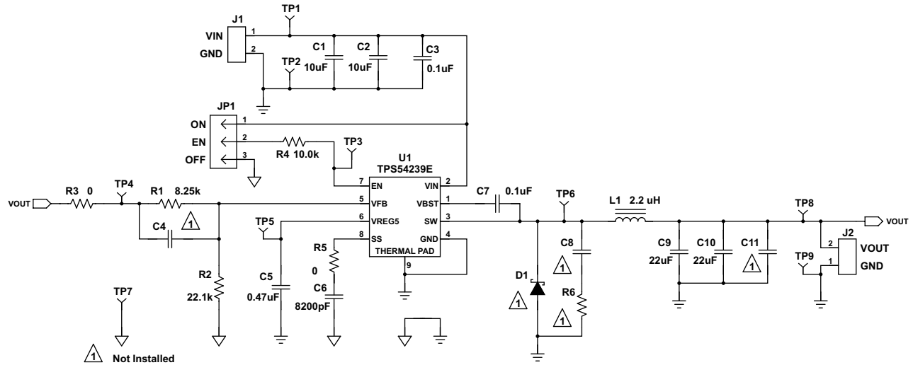
Figure 19. TPS54239EEVM-056 Schematic Diagram
