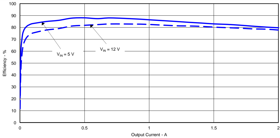
Figure 1. TPS54239EEVM-056 Efficiency
