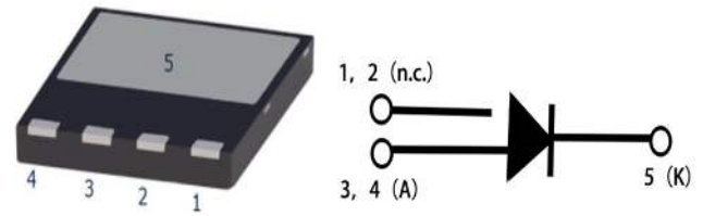
Bottom view
