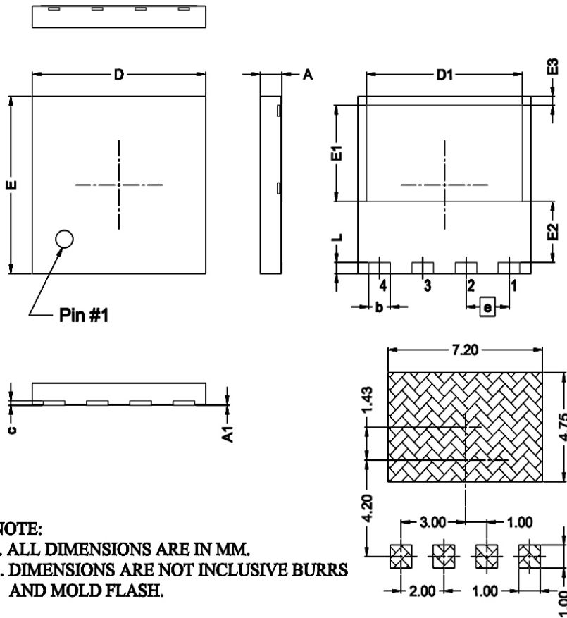
Land Pattern
