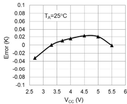
Normalized Error vs. Supply Voltage
