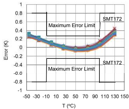
Accuracy vs. Temperature (TO18 V_{CC}=5\text{V} )
