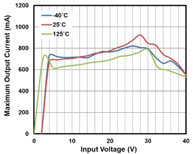
Figure 8. Output Current vs. Input Voltage
