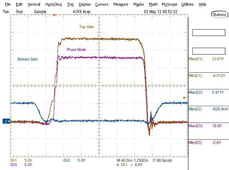
Figures 7 and 8: Switch Node Waveforms for V_{drr} = 5\text{ V}
