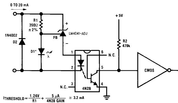
FIGURE 10. Simple Floating Current Detector
