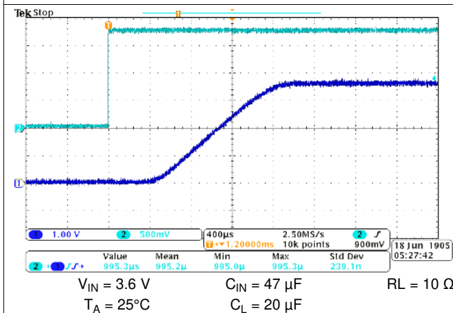
Figure 22. Turn-On Response
