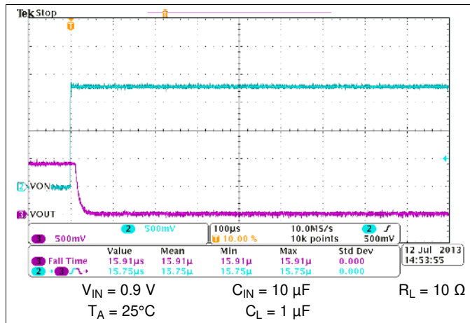
Figure 36. Turn-Off Response
