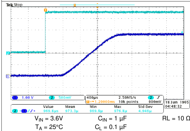
Figure 20. Turn-On Response
