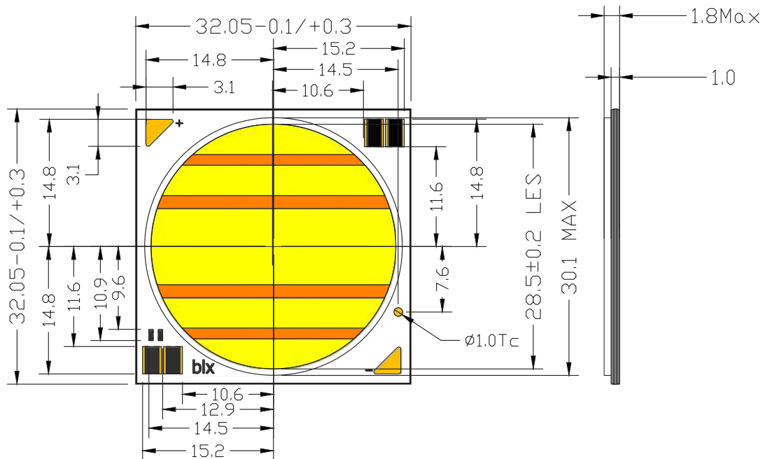
Figure 12: Mechanical Drawing Specification
