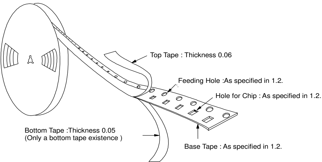
Fig.3 Taping Diagram
